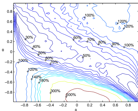
Figure 4: Contour plot of the simulated asymptotic relative efficiency of Schmid's estimator (cf. (13)) over Zhang's estimator (cf. (12)) for a stationary ARMA(1,1) process.
