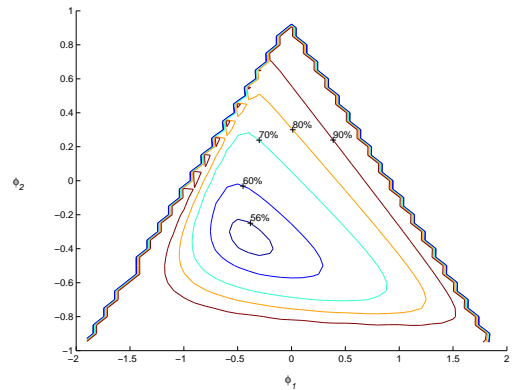
Figure 2: Contour plot of the asymptotic relative efficiency of Vermaat's estimator (cf. (14)) over Zhang's estimator (cf. (12)) for a stationary AR(2) process.
