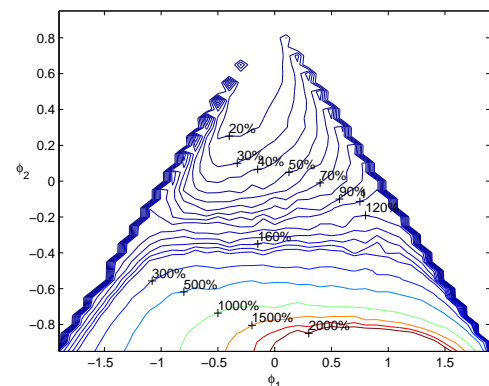
Figure 5: Contour plot of the simulated asymptotic relative efficiency of Schmid's estimator (cf. (13)) over Zhang's estimator (cf. (12)) for a stationary AR(2) process.
