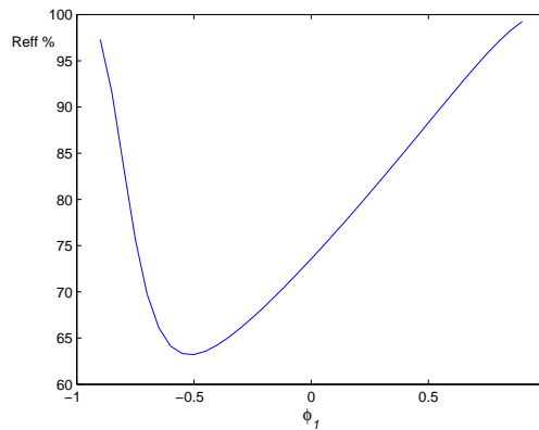
Figure 3: Plot of the asymptotic relative efficiency Schmid's estimator (cf. (13)) over Vermaat's estimator (cf. (14)) for a stationary AR(1) process.
