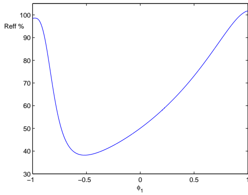
Figure 1: Plot of the asymptotic relative efficiency of Schmid's estimator (cf. (13)) over Zhang's estimator (cf. (12)) for a stationary AR(1) process.
